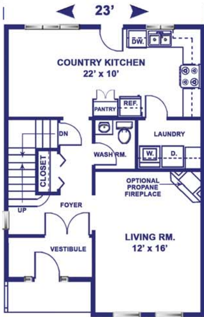
Main Floor Plan 723 Sq. Ft.
