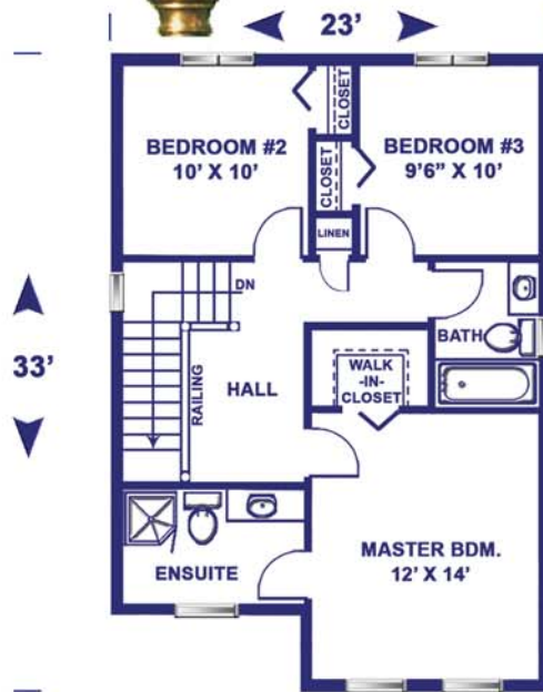
Second Floor Plan 723 Sq. Ft.
